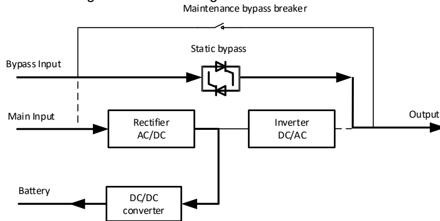
Figure 2-6 Bypass mode schematic diagram
