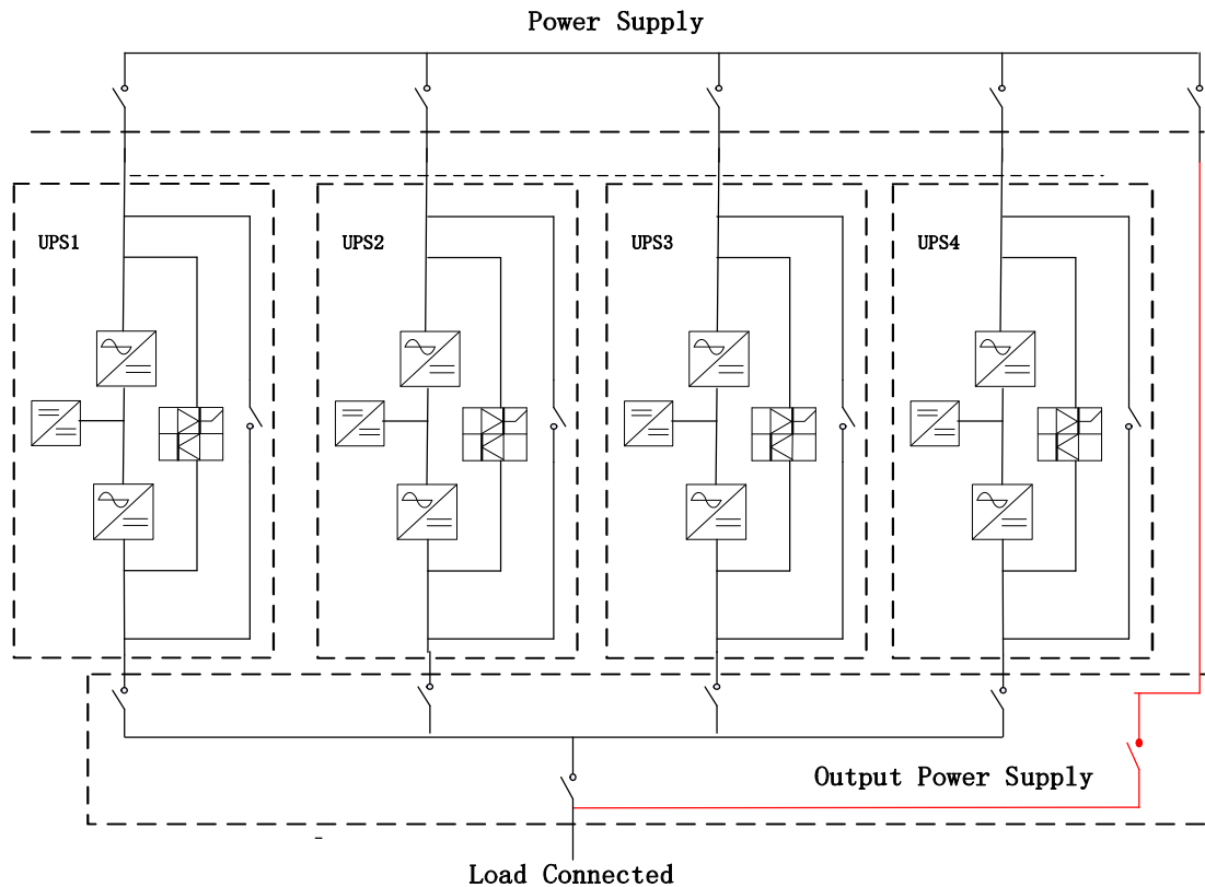
Figure5-3 Parallel Structure
