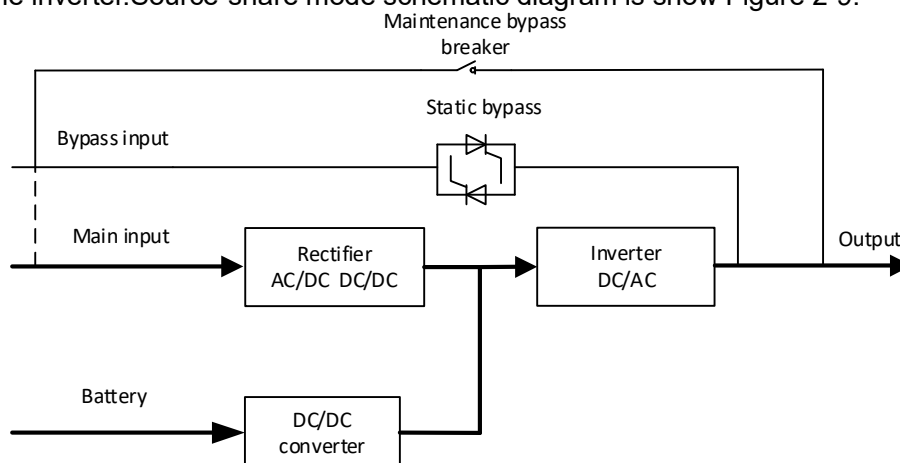
Figure 2-9 Source-share mode
